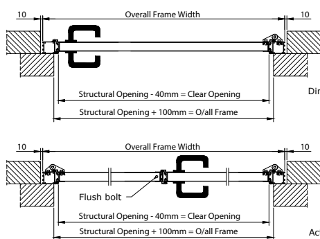
Installation behind the soffit, only inward opening
