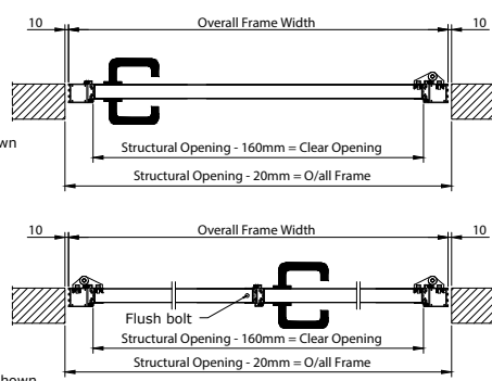
Installation within the soffit, inward or outward opening
